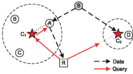
Fig. 2. The big picture of intentional caching.
